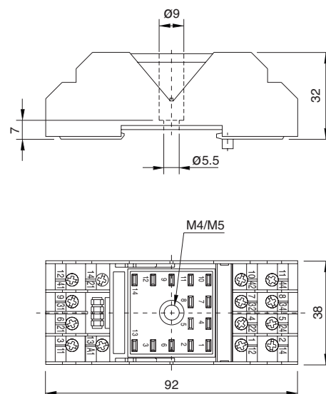
fig. 2. Dimension (mm)
